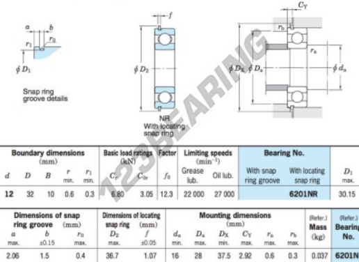
Single-row deep groove ball bearings ————— Koyo snap ring groove type locating snap ring type
